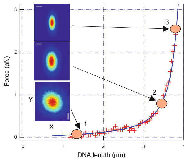
Fig. 2 Experimental extension curve data (crosses) fitted to the WLC model (blue solid line). The fitting gives the expected contour length ( L_0 ) of 4.1 μm, and persistence lengths ( P ) that vary between 47 and 57 nm for different measurements. Error bars are calculated to be far less than the size of the plotting symbols and are therefore not shown. The PSD measurements were done for the free bead (1) and for two states of molecular extension (2) and (3). The insets show histograms of the bead position in the xy plane, perpendicular to the beam propagation direction, with white lines indicating the scale (25 nm). We studied the histograms of the free bead and then, obtaining the trapping potential, we found that it was parabolic in the range of \pm 400 nm
