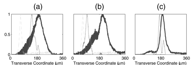
Fig. 3. Direct comparison between the output of the tandem and of a bulk crystal. Input (dashed) and output (solid) slices of the intensity profiles of the (a) FF( o ), (b) FF( e ), and (c) SH in the bulk (thick curves) and tandem (thin curves) samples. Intensity is normalized to the maximum value in all the cases. The relative position of the beams in the plot was chosen for easy comparison but does not correspond to the beam locations. Input energy: 15 \mu\text{J} ( \sim 60 \text{ GW/cm}^2 ).
