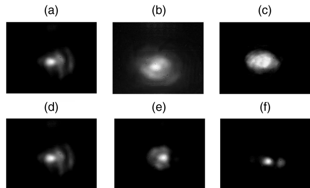
Fig. 2. Light output of the optical tandem under conditions of optimally phase-matched upconversion at low powers. (a), (d), FF( o ); (b), (e), FF( e ); (c), (f), SH. Input energy: top row, 2 \mu\text{J} ( \sim 7 \text{ GW/cm}^2 ); bottom row 15 \mu\text{J} ( \sim 60 \text{ GW/cm}^2 ). Input beam waist: \approx 18 \mu\text{m} .
