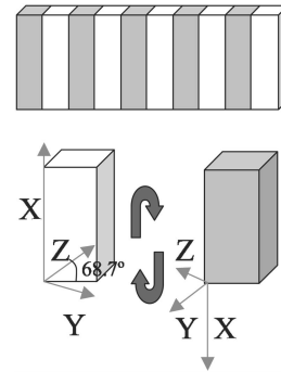
Fig. 1. Crystallographic topology of the optically contacted, walk-off-compensating KTP tandem. See text for full details.
