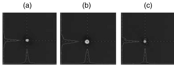
Fig. 4. Light output from the tandem in downconversion. (a) FF(o), (b) FF(e), (c) SH. Input intensity: SH pump, 46 \text{ GW/cm}^2 ; FF(o + e) seed, 0.6 \text{ GW/cm}^2 . Input waist of pump and seed beams: \approx 27 \mu\text{m} . A beam waist larger than in upconversion was used to reduce the strength of TPA at 532 nm.
